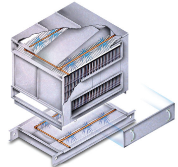
Precise humidity control and heat recovery systems for printing plants can help achieve annual energy savings of over $80,000 per year.
